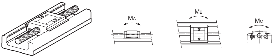
With a single short type block (Model KR-C)
