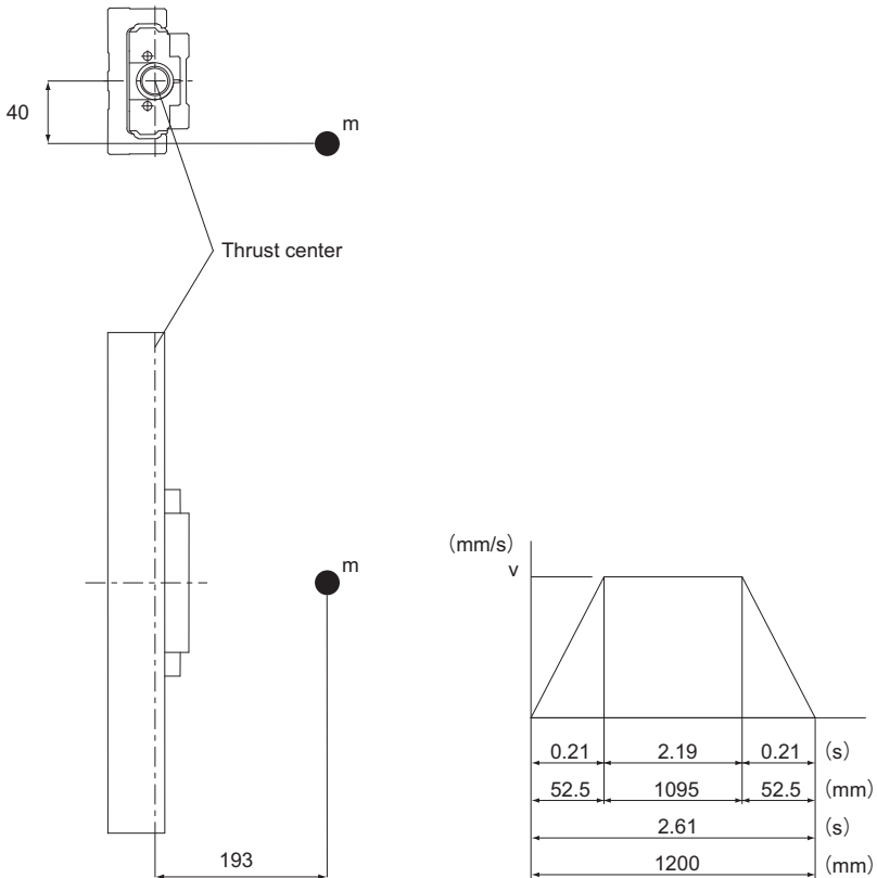
Fig.2 Velocity Diagram
