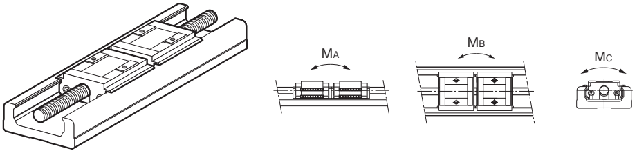
With double short type blocks (Model KR-D)
