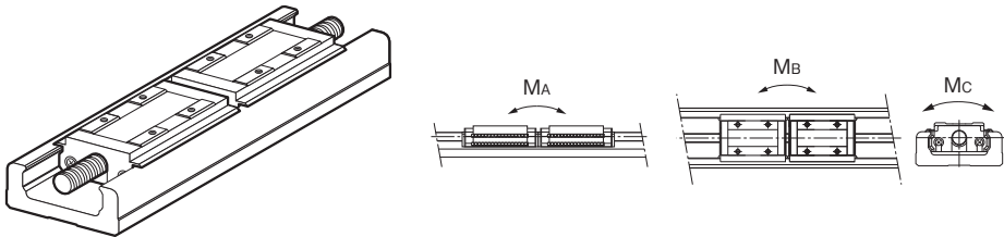
With double long type blocks (Model KR-B)
