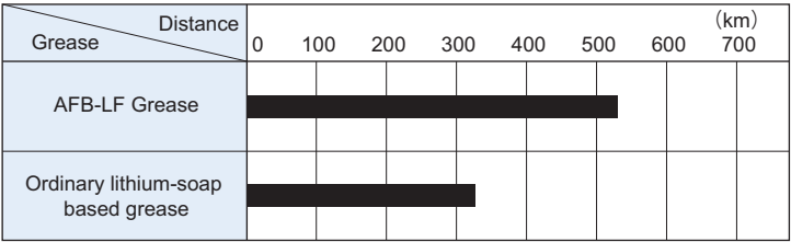
Travel distance until flaking occurs by grease type
